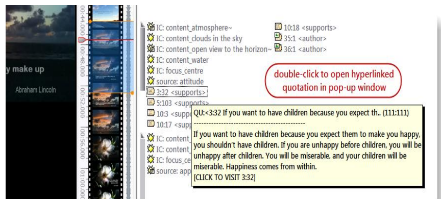
Figure 319: Traversing hyperlinks
